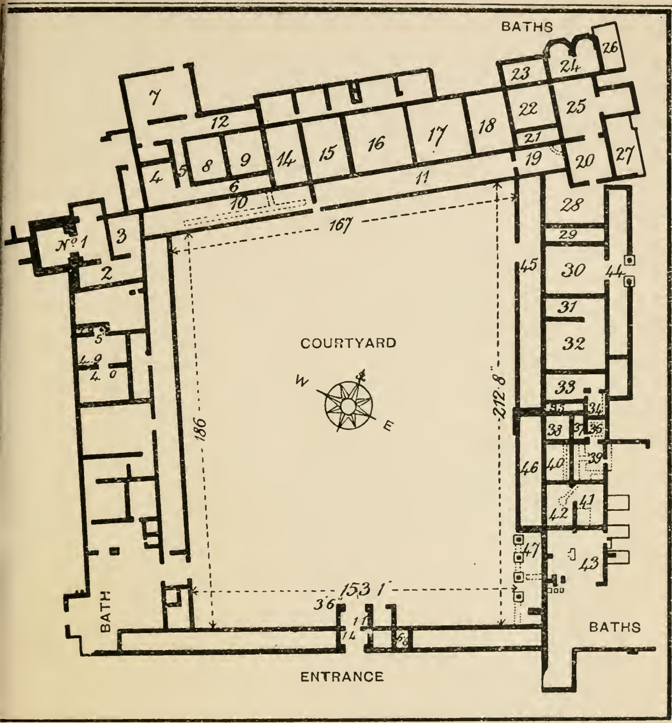
FIG. 11. COURTYARD HOUSE AT NORTBLEIGH, OXFORDSHIRE, AS EXCAVATED IN 1815-16. Room 1, chief mosaic with hypocaust; rooms 8-18, mosaic floors; rooms 21-7 and 38-43, baths, &c.; the west wing had poorer rooms, perhaps for servants. Recent excavations show that this plan represents the house in its third and latest stage; in the corridor (10) a part of the earlier house-front is shown by dotted lines. The pottery found in the recent excavations suggests that the first house on this spot was built not later than the early second century.
