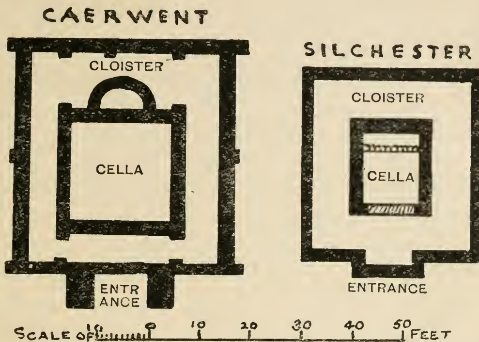
FIG. 9. TWO GROUND-PLANS OF ROMANO-BRITISH TEMPLES.
